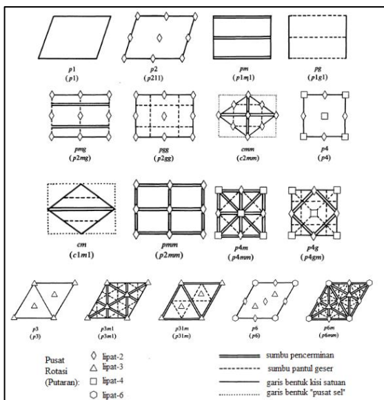
Figure 1. Crystallographic Pattern (Liu & Collins, 1998)
